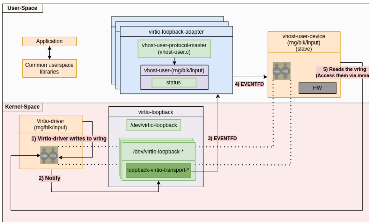
Figure 11: virtio-driver sends data to vhost-user-device : After having written new data in the vrings , the virtio-driver notifies the vhost-user-device to read it via the virtio-loopback-transport driver by executing the notify function which is defined by the virtio-loopback-transport driver (Step 1-2). Such function triggers an eventfd to the virtio-loopback-adapter , and the last another eventfd to the vhost-user-device , that will know at that point that new data has been written in the vrings shared memory (Step 3-5).
