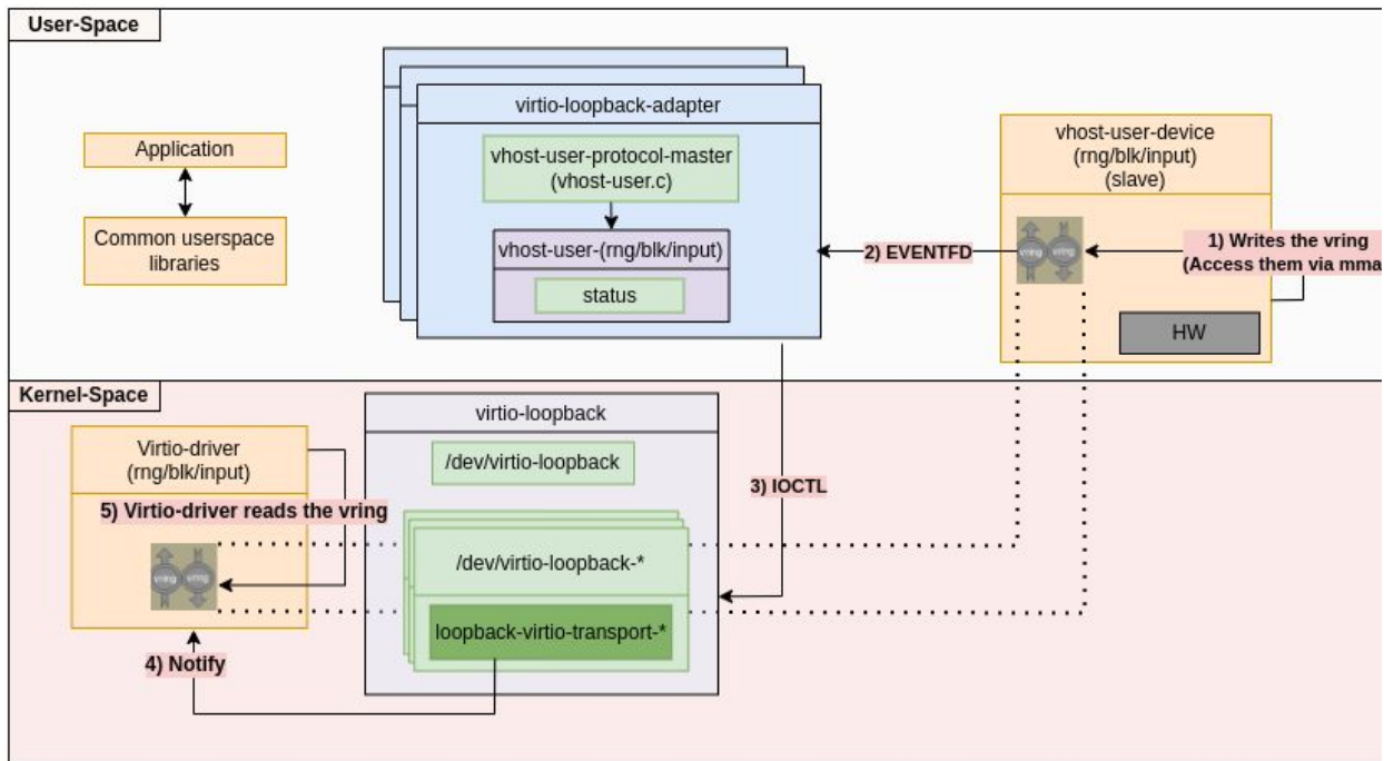
Figure 12: virtio-driver receives data from vhost-user-device : After having written the vrings memory, the vhost-user-device notifies the virtio-loopback-adapter with an eventfd and the last delivers this notification to the loopback driver via an ioctl/write call(Step 1-3). At this point, as a result of the SYS_CALL, the virtio-loopback-transport notifies (by calling the function “vm_interrupt”) the virtio-driver to read the vrings (Step 3). Finally, the virtio-driver reads the new data from the vrings (Step 4). This is an optimized execution flow that will be evaluated from the viewpoint of the impact it has on the existing device implementation. The alternative is to pass by the virtio-loopback adapter.
